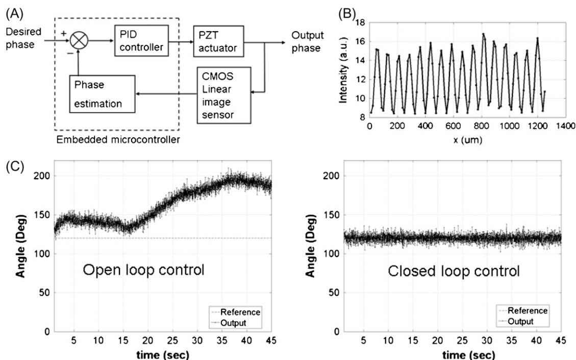
FIGURE 3 SW phase control with closed loop feedback controller. (A) Schematic diagram of the SW phase closed loop control unit. The embedded microcontroller monitors the output phase from the CMOS detector and this estimated phase is used to control input in real time ( \sim 70 Hz). (B) Typical fringe pattern on CMOS image sensor. The invisible evanescent SW on the sample can be indirectly monitored in this alternative way. (C) SW fringe phase measurement with a feedback loop open (left) and closed (right). Reference angle: 120^\circ and measurement duration: 0.2–45 s. The standard deviation of the fluctuation is <3^\circ .
